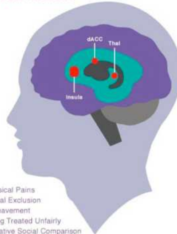
Pain Network
