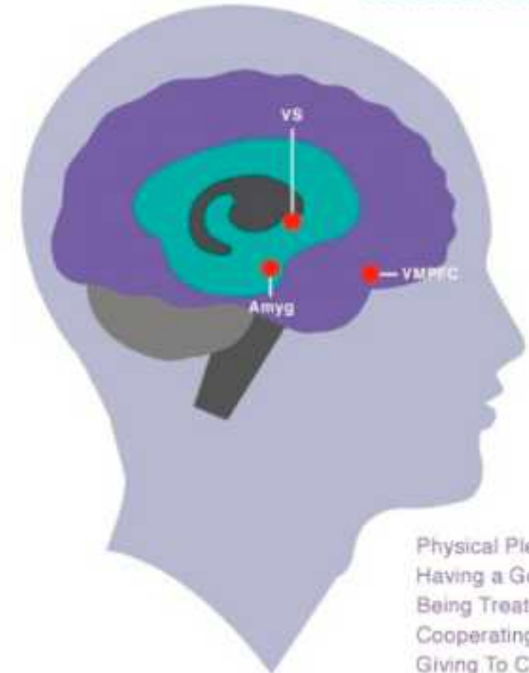
Reward Network
